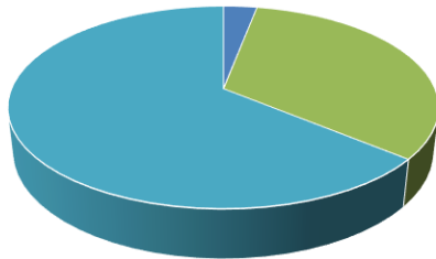
GHG emissions in the EU28 in 2017
